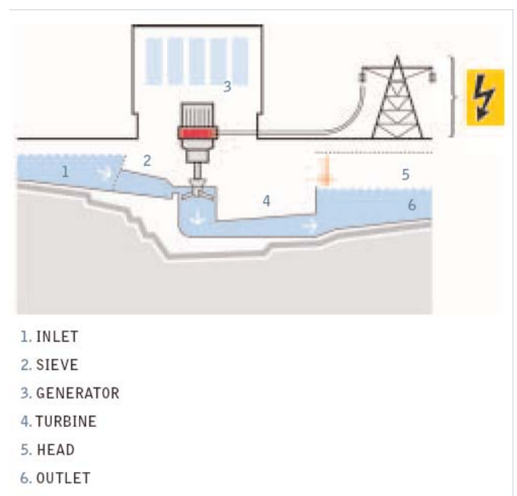
figure 39: hydro technology
