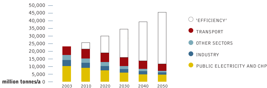
figure 27: development of global CO 2 emissions by sector under the energy [r]evolution scenario
