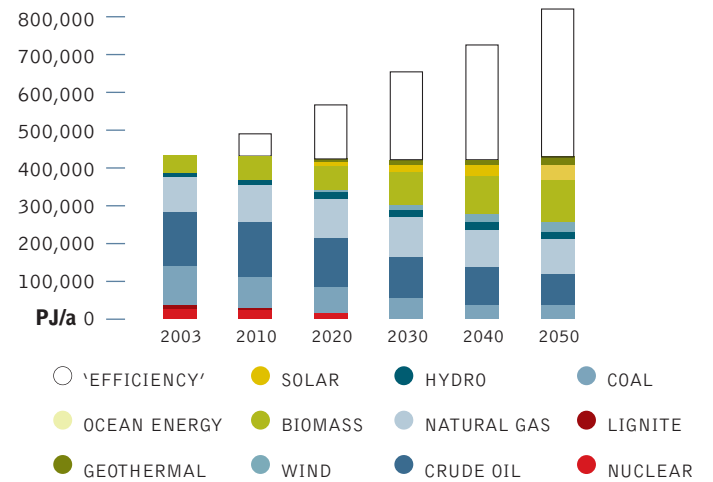
figure 26: development of global primary energy consumption under the energy [r]evolution scenario
