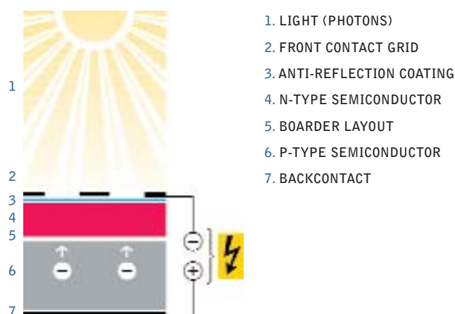
figure 31: photovoltaics technology
