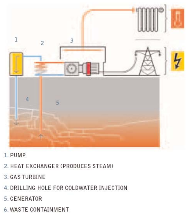
figure 38: geothermal technology
